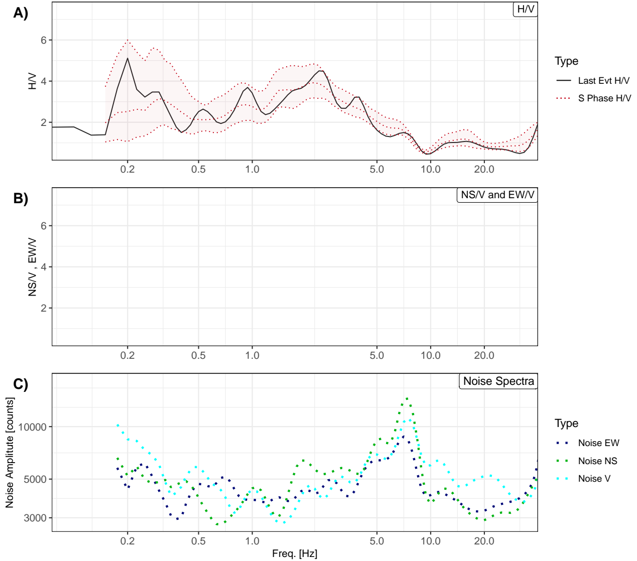
H/V and noise spectra. Spectral ratios are computed considering both S-phase and noise windows, as indicated in the legend. A) H/V for the horizontal (H) component, the average \pm one standard deviation of the ratios computed for several windows are also shown and the gray line (Figure A) is the H/V relative to the last automatically processed seismic event. B) H/V for the EW and NS components (mean). C) noise spectra (mean).
